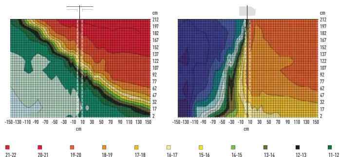
Opening without air curtain.
