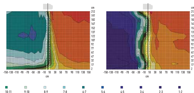
Opening with air curtain, too high speed.
